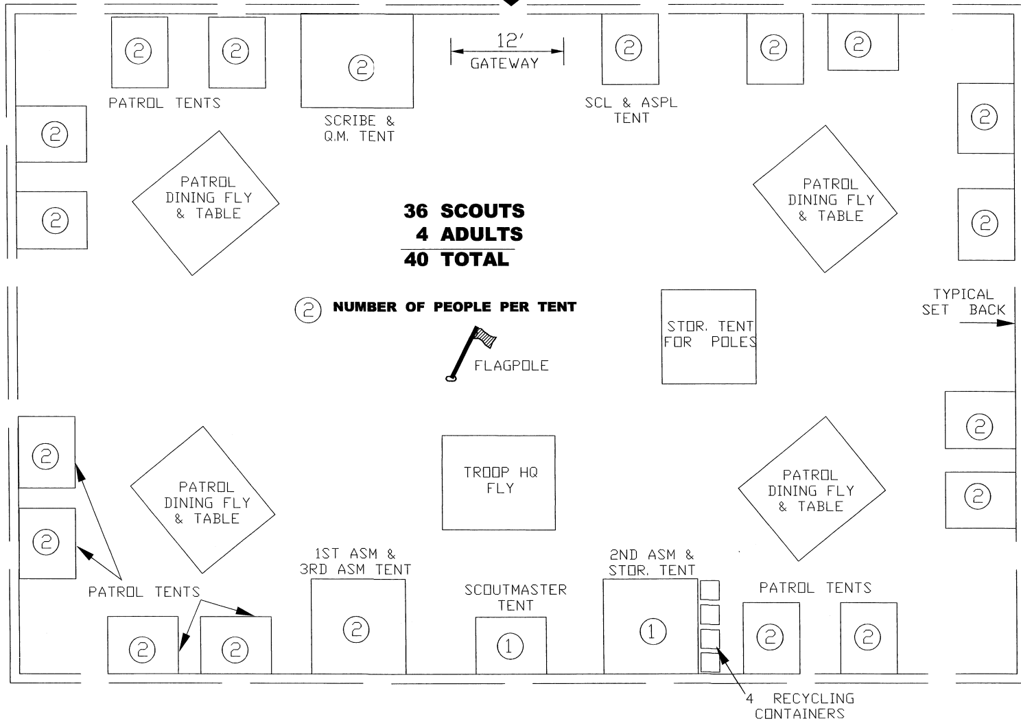
TYPICAL TROOP SITE (APPROX. 8000 SQ. FT.)
